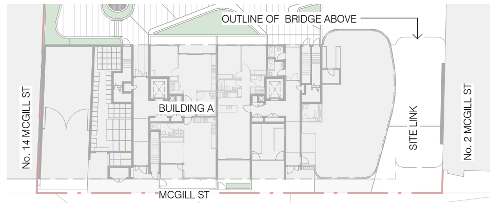
LEVEL GROUND
