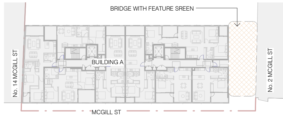
LEVEL 02 - 05
